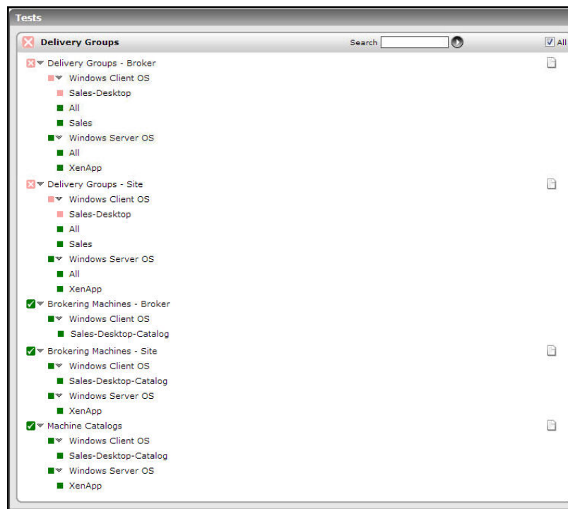
Figure 8.11: The Delivery Groups layer
