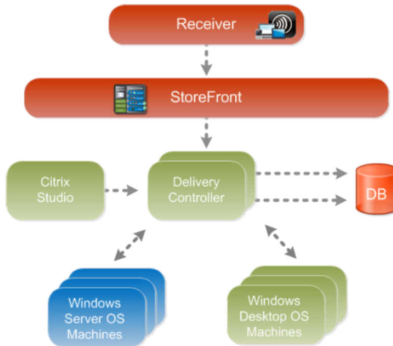
Figure 8.1: The Delivery Controller 7 architecture
