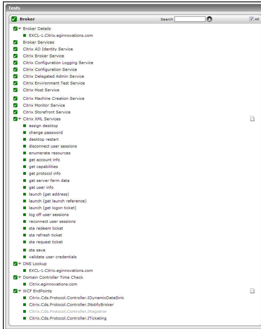
Figure 8.9: The tests mapped to the Broker layer
