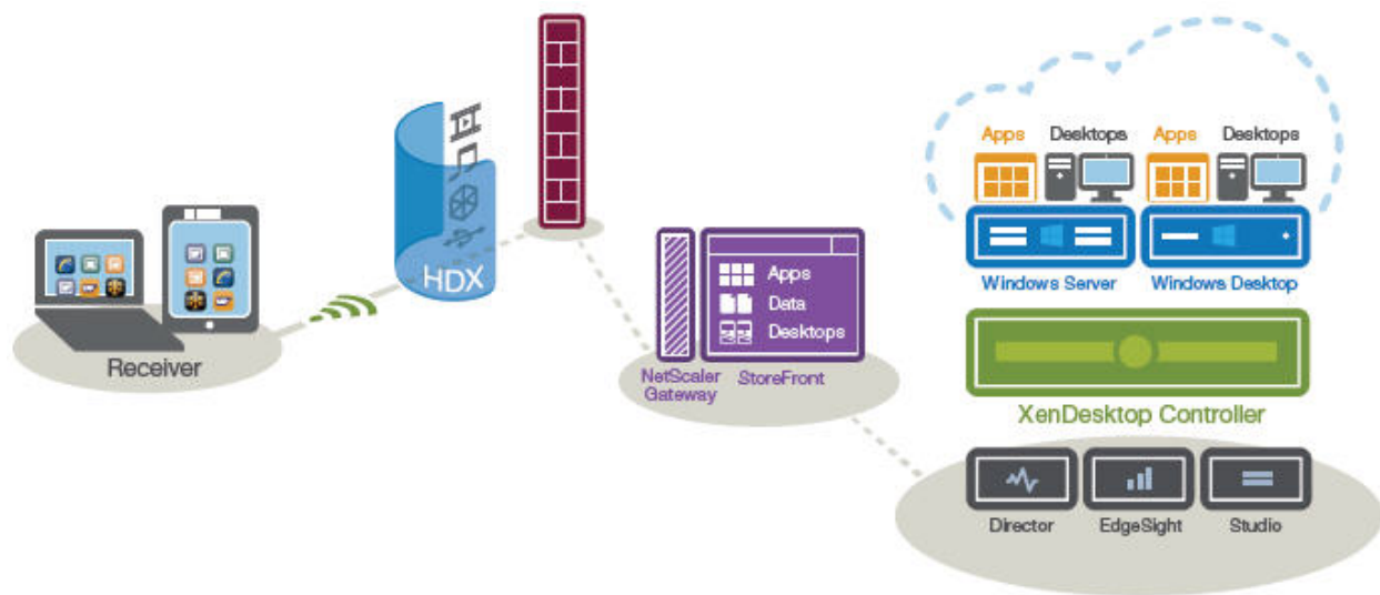
Figure 8.2: The Delivery Controller 7 architecture
