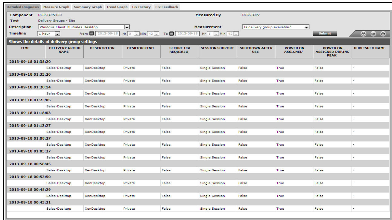
Figure 8.18: The detailed diagnosis of the Is delivery group available? measure
