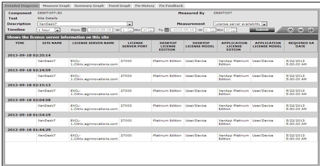
Figure 8.7: The detailed diagnosis of the License server availability measure
