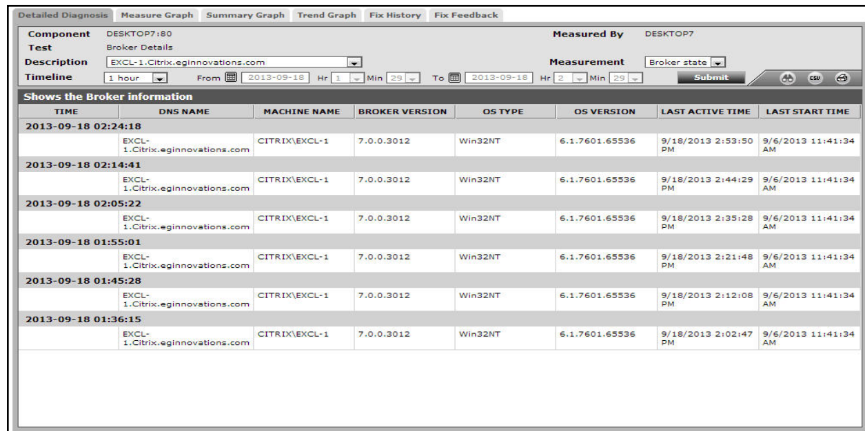
Figure 8.10: The detailed diagnosis of the Broker state measure
