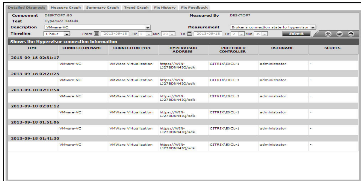
Figure 8.5: The detailed diagnosis of the Broker's connection state to hypervisor measure
