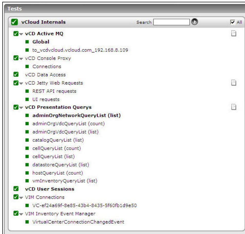
Figure 3.2: The tests mapped to the vCloud Internals layer
