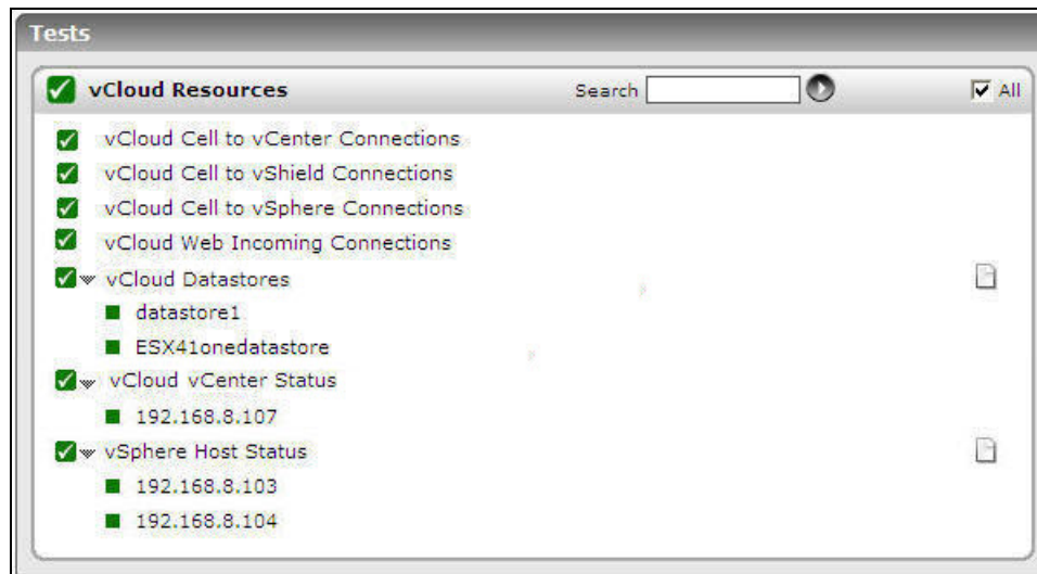
Figure 3.4: The tests mapped to the vCloud Resources layer
