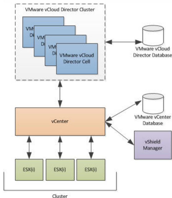
Figure 1.1: Architecture of the vCloud Director
