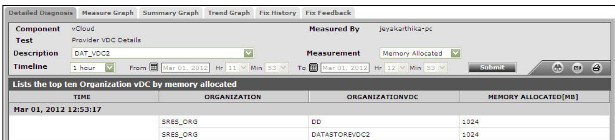
Figure 3.9: The detailed diagnosis of the Memory Allocated measure
