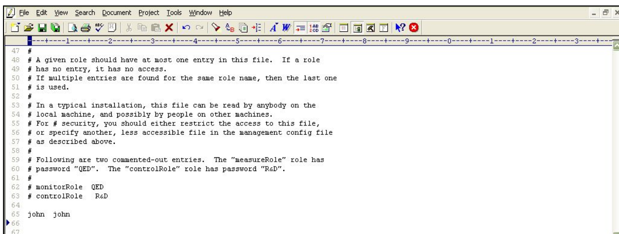
Figure 2.5: Appending a new username password pair
