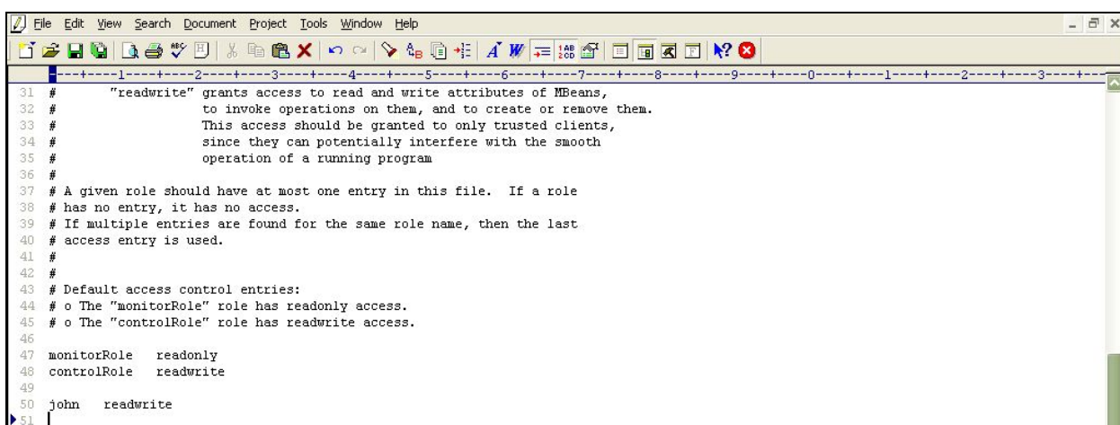
Figure 2.6: Assigning rights to the new user in the jmxremote.access file
