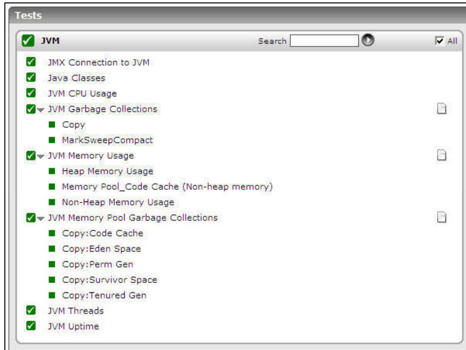
Figure 2.2: The tests mapped to the JVM layer
