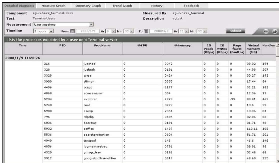
Figure 3.7: The detailed diagnosis of the User sessions measure
