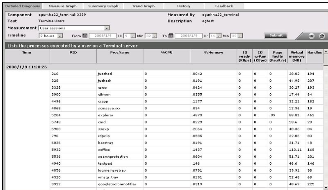
Figure 3.11: The detailed diagnosis of the User sessions measure
