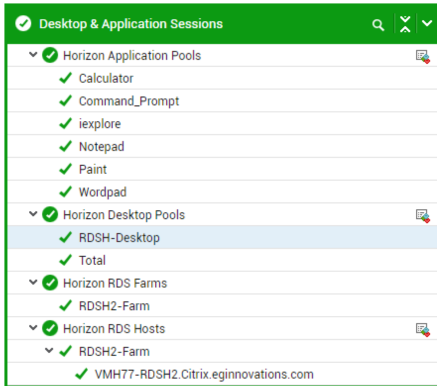
Figure 3.4: The test mapped to the Desktop and Application Sessions layer
