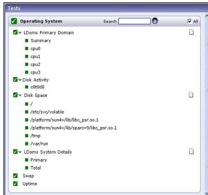
Figure 3.2: The tests mapped to the Operating System layer
