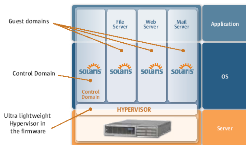
Figure 1.1: The architecture of a Solaris LDoms server
