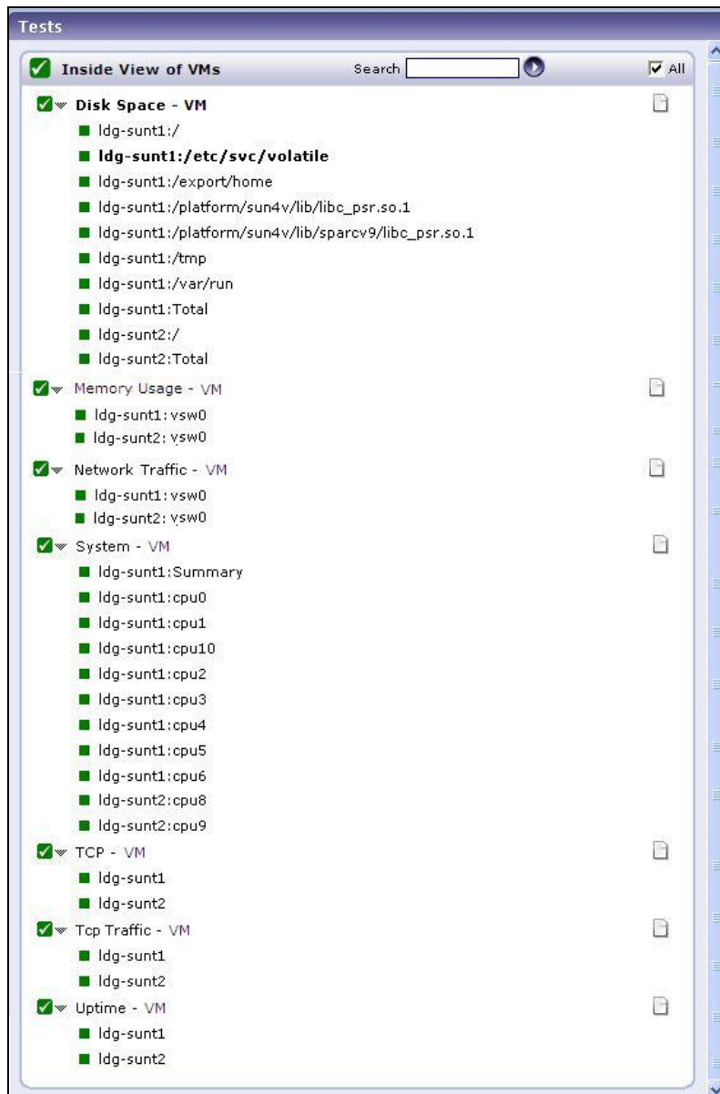
Figure 3.9: The tests associated with the Inside View of VMs layer
