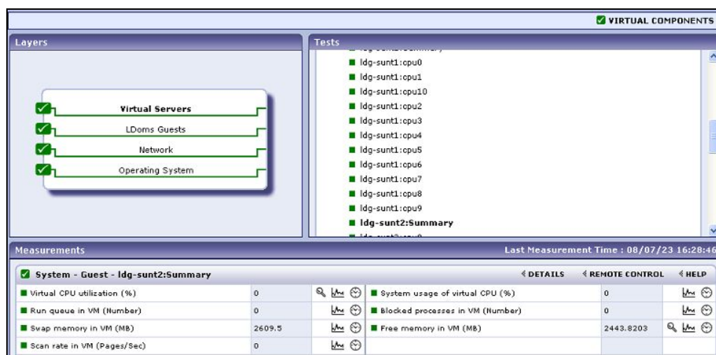
Figure 3.10: The tests mapped to the Virtual Servers layer
