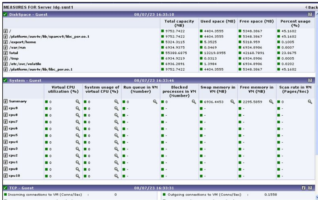
Figure 3.11: Measures pertaining to a chosen guest
