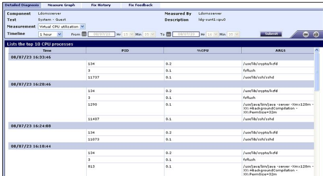
Figure 3.17: The top 10 CPU consuming processes
