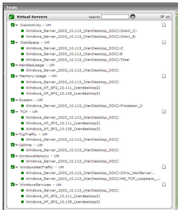
Figure 3.15: The tests associated with the Inside View of VMs layer
