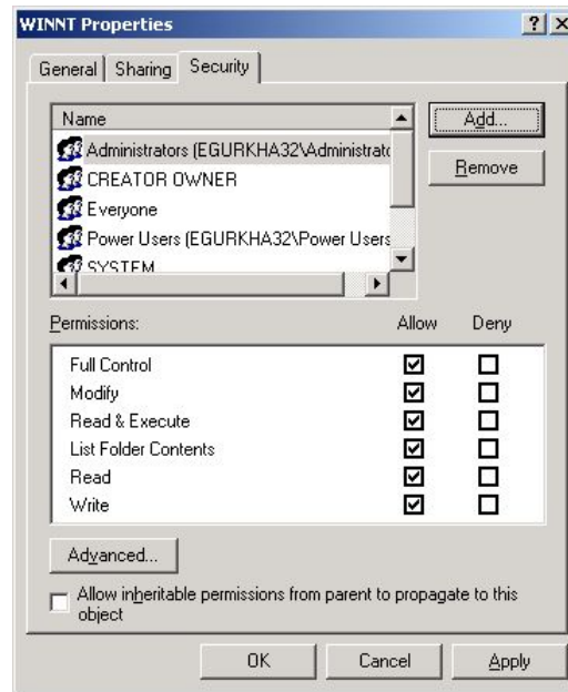
Figure 2.10: Defining the Security settings for the ADMIN$ share
