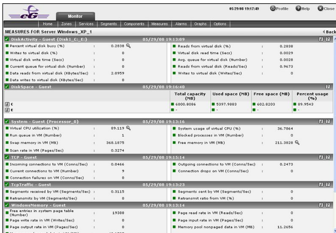
Figure 3.33: Measures pertaining to a chosen guest
