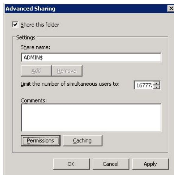
Figure 2.15: Enabling the ADMIN$ share
