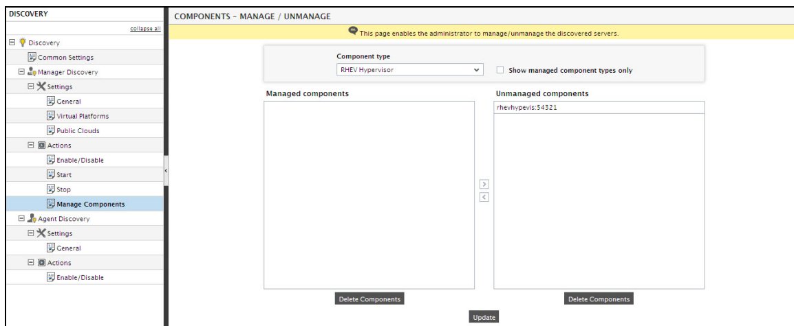
Figure 2.55: Viewing unmanaged RHEV Hypervisors
