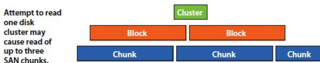
Figure 3.11: Unaligned partitions
