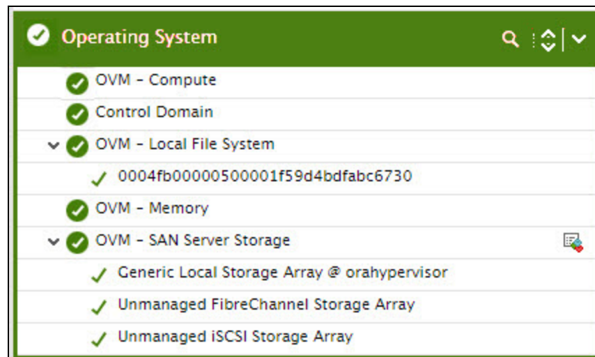
Figure 3.2: The tests mapped to the Operating System layer
