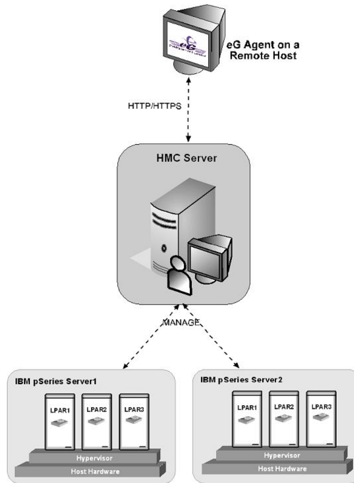
Figure 2.1: How the eG single agent monitors an IBM pSeries Server
